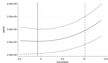
(c) Lasso CV function for interaction design
