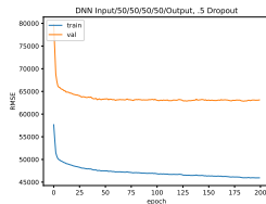
(B) dropout
